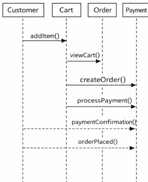
Sequence Diagram 1: Place Order
